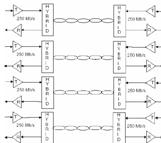
Figure 40-2—1000BASE-T topology
