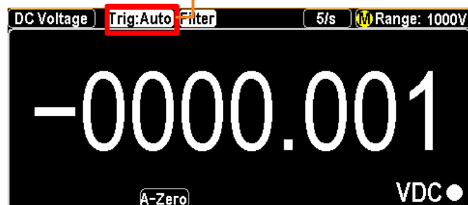
Indicator Auto (Internal) Trigger Mode
