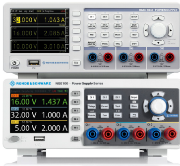
R&S®HMC8043 and R&S®NGE100B three-channel power supply
