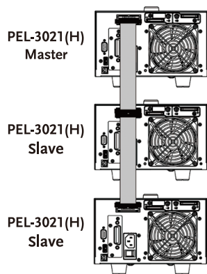
3台PEL-3021(H)并联
